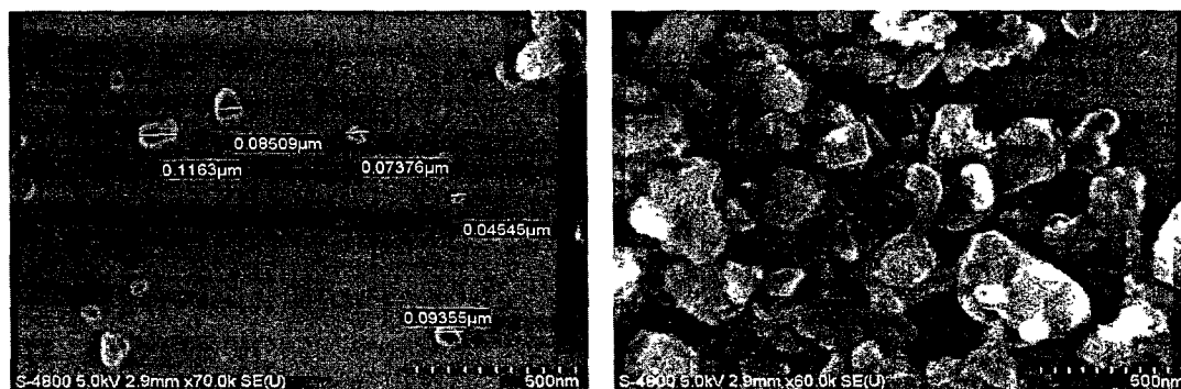
Figure 4-4 SEM image of the formed curcumin nanoparticles (left) diluted sample, and (right) concentrated sample
