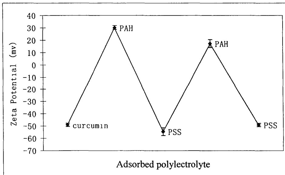
Figure 5-2 Particle \xi -potential alternation during LbL coating of curcumin (pH 6.5) Standard deviation shows the same sample run 10 times on zeta potential analyzer
