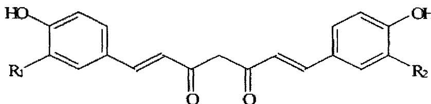
Figure 4-2 Structural formula for curcumin
